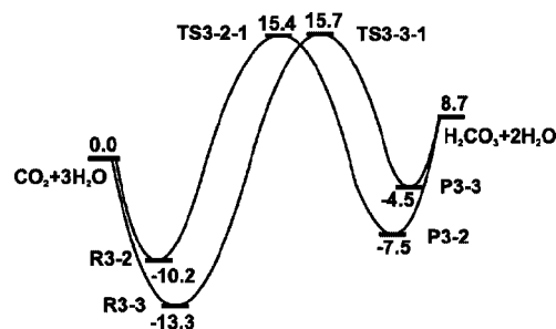
Figure 7. Potential energy profiles for two channels of the \text{CO}_2 + 3\text{H}_2\text{O} addition reaction at 0 K. Relative energies given in kcal/mol obtained from calculated heats of formation.
